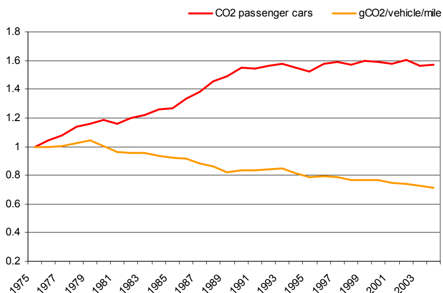
Figure 11: CO 2 emissions from passenger cars from 1975 to 2004 ('000 tonnes)
